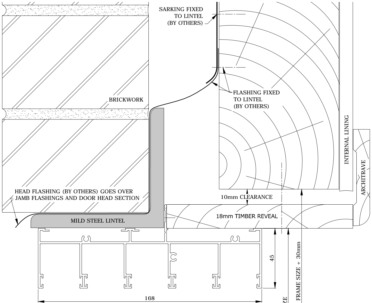
HEAD DETAIL
