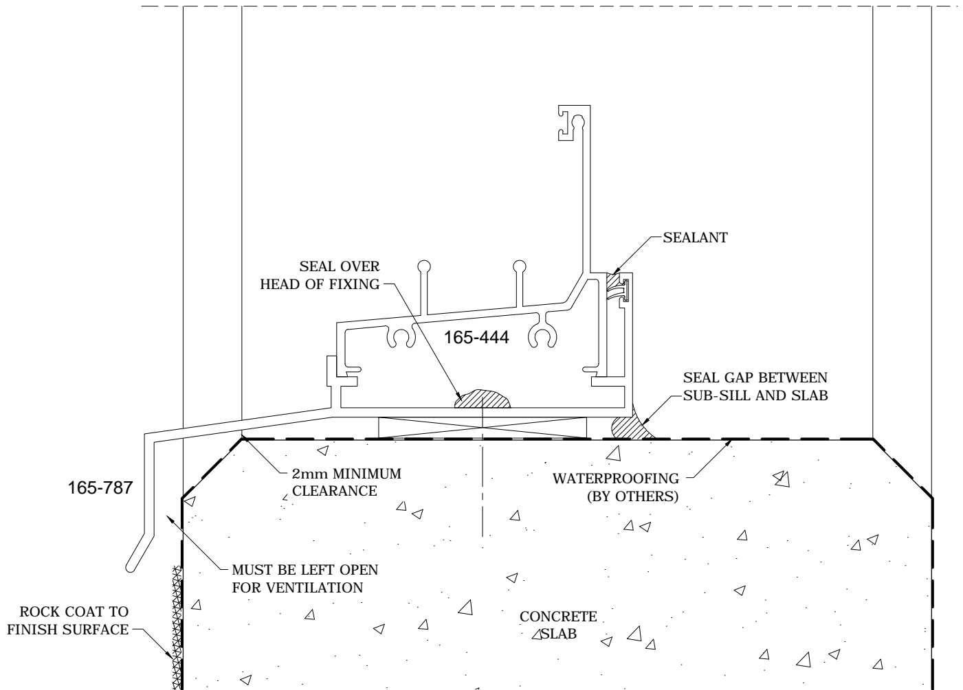
SILL DETAIL
