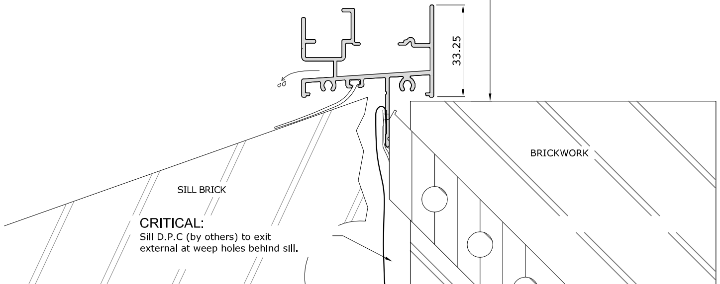
DETAIL 2 of 3 SILL
